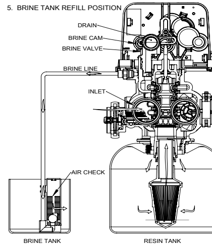
5. BRINE TANK REFILL POSITION
